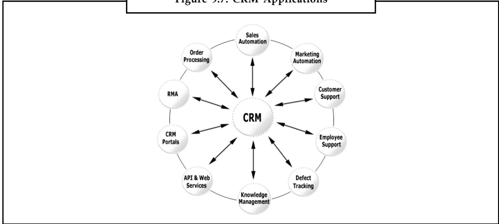
Figure 9.7: CRM Applications
