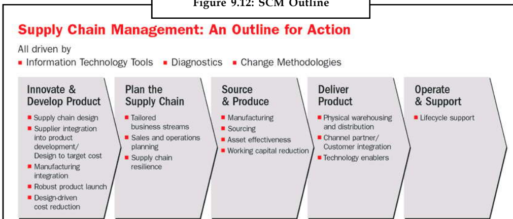
Figure 9.12: SCM Outline
