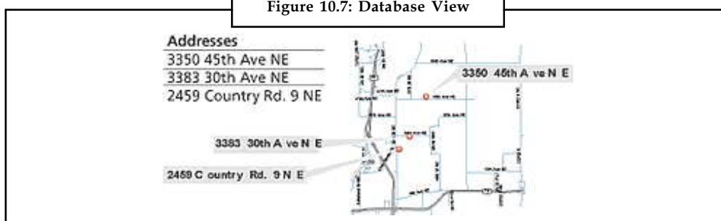
Figure 10.7: Database View
