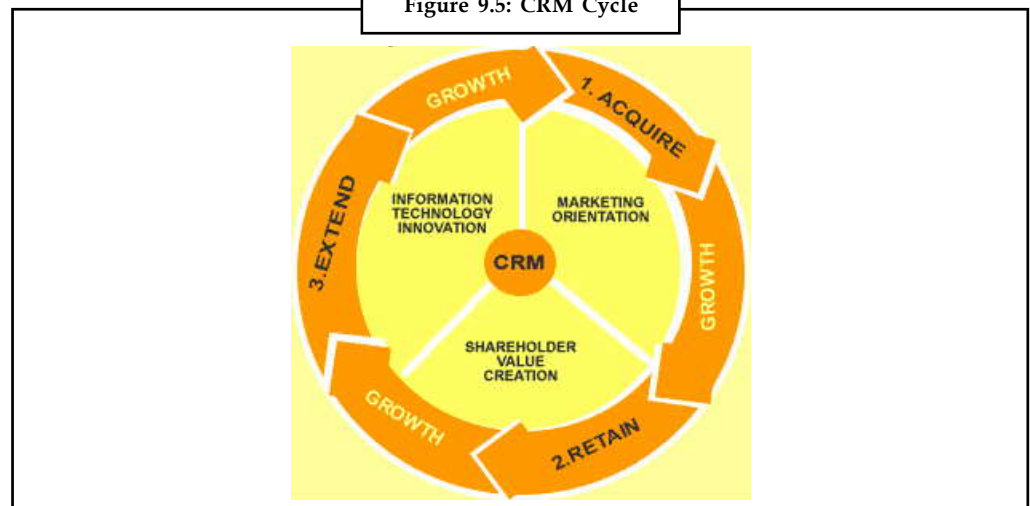
Figure 9.5: CRM Cycle
