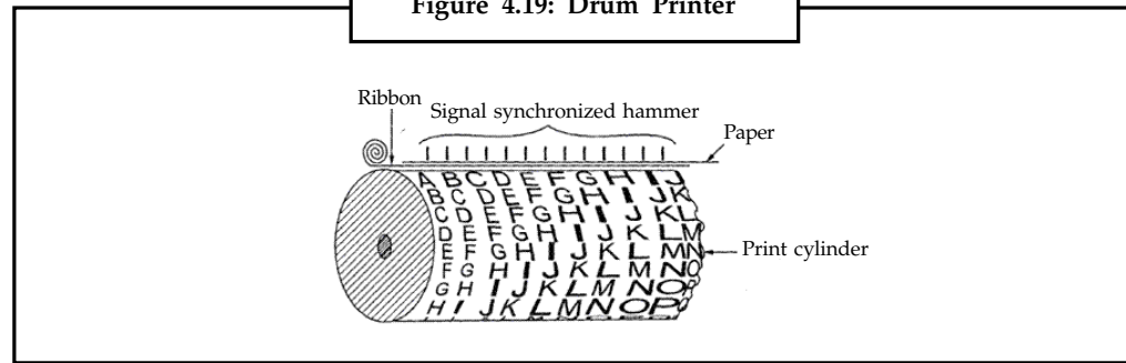
Figure 4.19: Drum Printer
