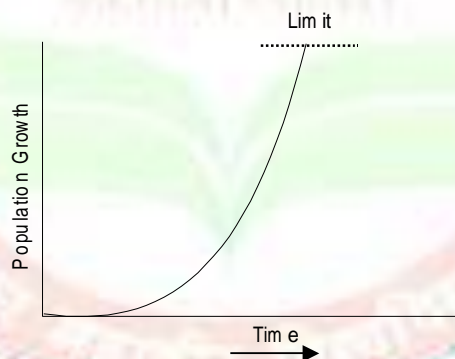
Figure 7.3. J-shaped growth curve.
