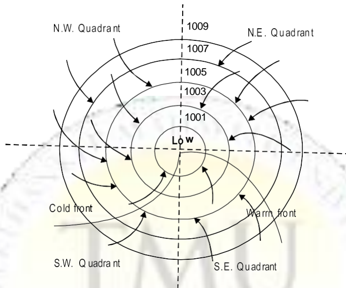
Figure 5.1: A generalized temperate cyclone in northern hemisphere.
